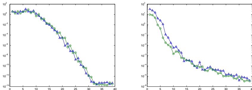
Figure 2: Uniform error (circles) and estimate (10) (triangles) of Newton interpolation at Discrete Leja Points on the square for \nu = 2, \dots, 40 ; Left: f(x_1, x_2) = \cos(5(x_1 + x_2)) ; Right: f(x_1, x_2) = [(x_1 - 1/3)^2 + (x_2 - 1/3)^2]^{5/2} .
