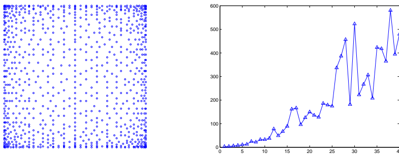
Figure 1: Left: N = 861 Discrete Leja Points for degree n = 40 on the square, extracted from an 81 \times 81 Chebyshev-Lobatto grid; Right: Lebesgue constants of Discrete Leja Points on the square for n = 1, \dots, 40 .
