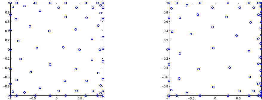
Figure 11: N = 66 approximate Fekete points of degree n = 10 in the real square of Example 5, with \varepsilon = 1 (left) and \varepsilon = 0.01 (right).
