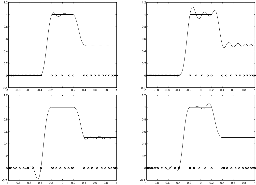
Figure 16: Multiband polynomial filters for K_1 = [-1, -0.4] , K_2 = [-0.2, 0.2] and K_3 = [0.4, 1] at approximate Fekete points of degree n = 30 : nonweighted (top-left), weights (100, 1, 1) (top-right), (1, 100, 1) (bottom-left), (1, 1, 100) (bottom-right); the small circles (o) indicate the approximate Fekete points.
