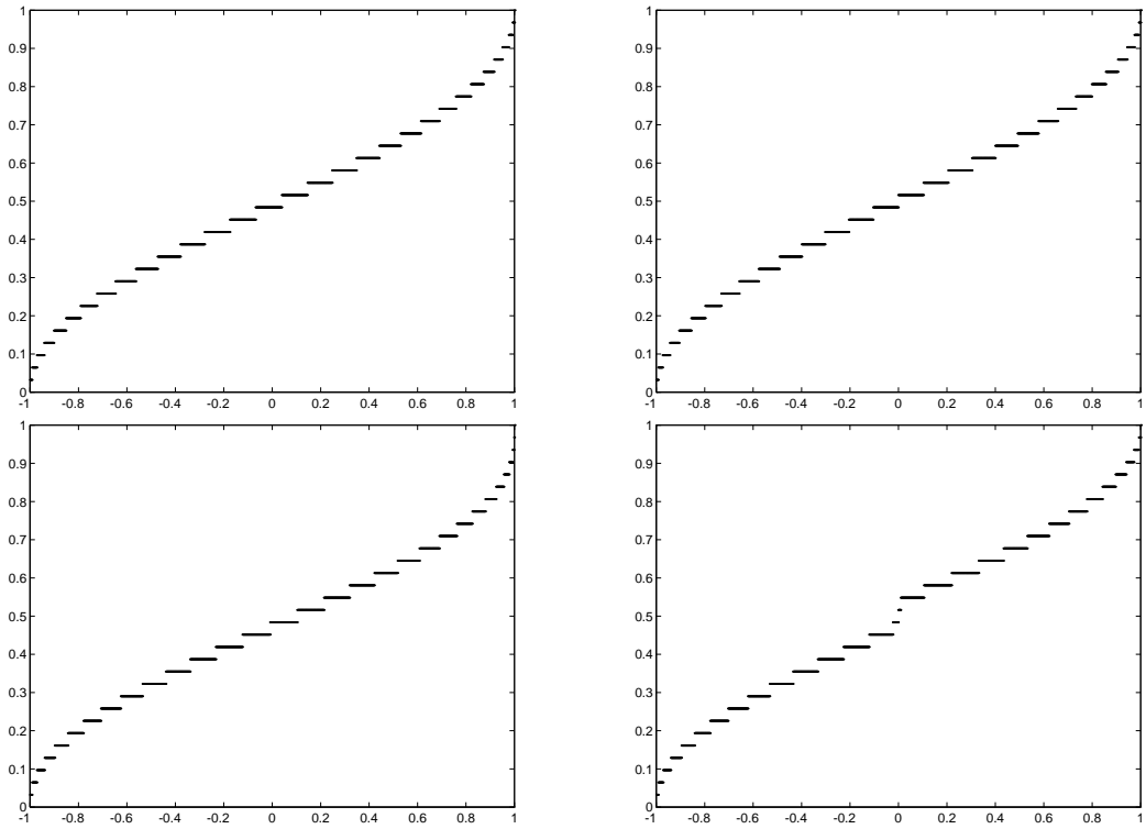
Figure 4: Distribution functions of N = 31 approximate Fekete points of degree n = 30 in Example 1 (left) and Example 2 (right), for \varepsilon = 1 (top) and \varepsilon = 0.01 (bottom).
