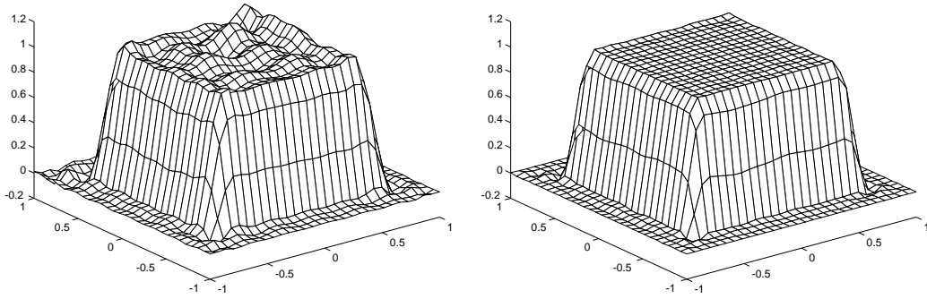
Figure 19: Nonweighted polynomial filters of degree n = 20 (left) and n = 30 (right) for Example 9-(39).
