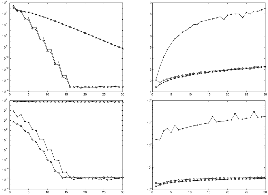
Figure 8: Interpolation errors (left) and Lebesgue constants (right) versus the interpolation degree, in Example 4 for \varepsilon = 1 (top) and \varepsilon = 0.01 (bottom); the interpolation spaces are \mathbb{P}_n with Fekete points for nonweighted polynomial interpolation (*), w_\varepsilon\mathbb{P}_n again with the latter points (+), w_\varepsilon\mathbb{P}_n with approximate Fekete points for weighted polynomial interpolation (o).
