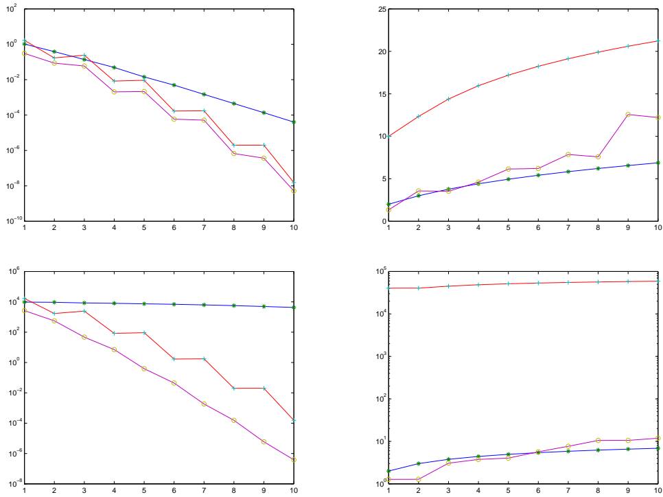
Figure 10: Interpolation errors (left) and Lebesgue constants (right) versus the interpolation degree, in Example 5 for \varepsilon = 1 (top) and \varepsilon = 0.01 (bottom); the interpolation spaces are \mathbb{P}_n with the Padua points for nonweighted polynomial interpolation (*), w_\varepsilon\mathbb{P}_n again with the latter points (+), w_\varepsilon\mathbb{P}_n with approximate Fekete points for weighted polynomial interpolation (o).
