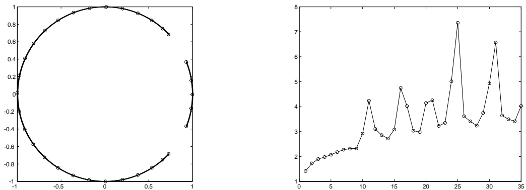
Figure 18: N = 32 approximate Fekete points of degree n = 31 for the complex low-pass weighted filter in Example 8 (left); Lebesgue constants versus the interpolation degree (right).
