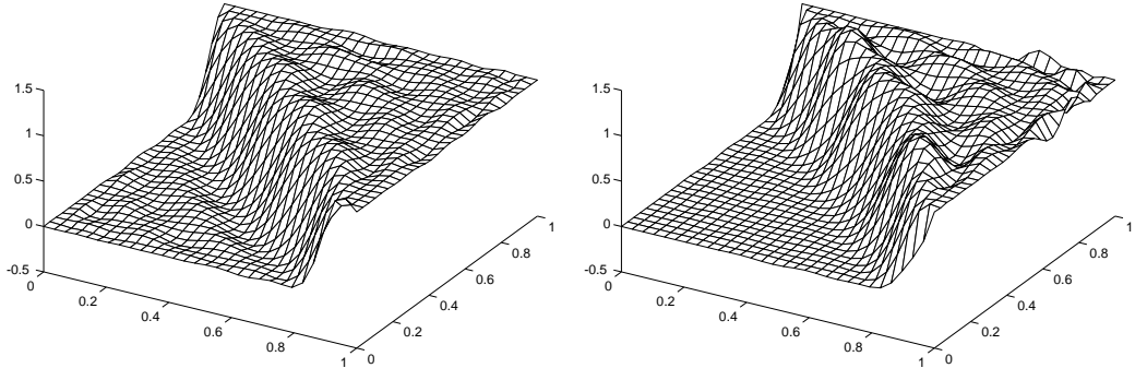
Figure 21: Two-dimensional filters of degree n = 20 for Example 9-(40) with w_1 = 1, w_2 = 1 (left) and w_1 = 10, w_2 = 1 (right).
