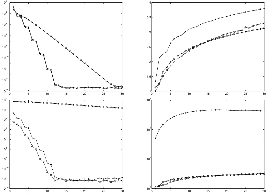
Figure 1: Interpolation errors (left) and Lebesgue constants (right) versus the interpolation degree, in Example 1 for \varepsilon = 1 (top) and \varepsilon = 0.01 (bottom); the interpolation spaces are \mathbb{P}_n with Chebyshev-Lobatto points (*), w_\varepsilon \mathbb{P}_n with Chebyshev-Lobatto points (+), w_\varepsilon \mathbb{P}_n with approximate Fekete points (o).
