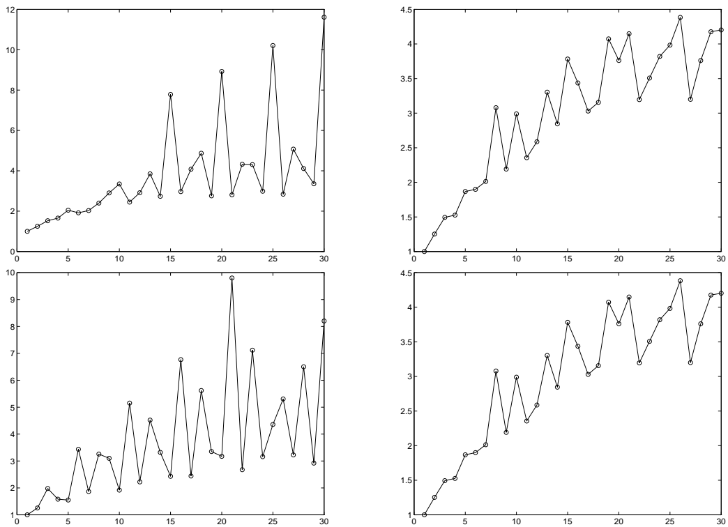
Figure 17: Lebesgue constants versus the interpolation degree for the multi-band filters above: nonweighted (top-left), weights (100, 1, 1) (top-right), (1, 100, 1) (bottom-left), (1, 1, 100) (bottom-right).
