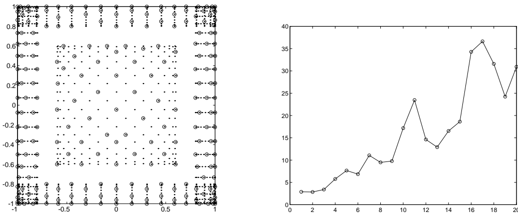
Figure 20: Left: N = 231 nonweighted approximate Fekete points (circles) of degree n = 20 extracted from a weakly admissible mesh (dots) for Example 9-(39). Right: estimated Lebesgue constants versus the interpolation degree for the same example.
