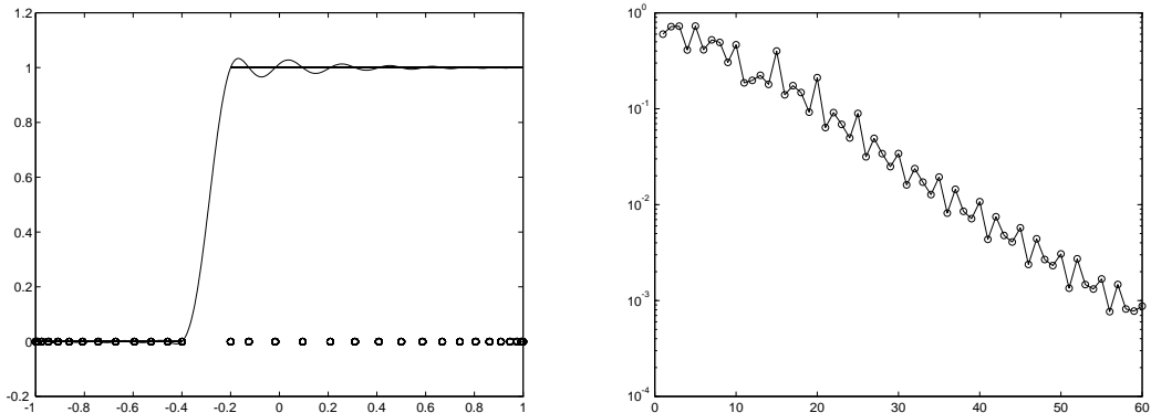
Figure 15: High-pass nonweighted polynomial filter for K_1 = [-1, -0.4] and K_2 = [-0.2, 1] of degree n = 30 (left), and interpolation errors up to degree n = 60 (right).
