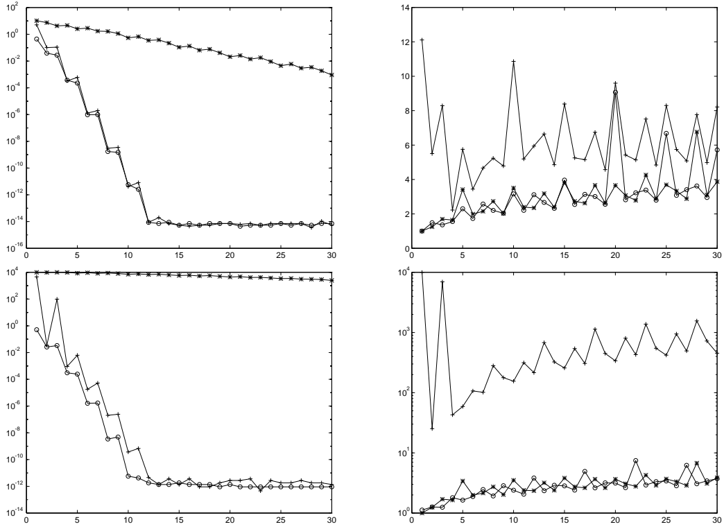
Figure 5: Interpolation errors (left) and Lebesgue constants (right) versus the interpolation degree, in Example 3 for \varepsilon = 0.3 (top) and \varepsilon = 0.01 (bottom); the interpolation spaces are \mathbb{P}_n with approximate Fekete points for nonweighted polynomial interpolation (*), w_\varepsilon\mathbb{P}_n again with the latter points (+), w_\varepsilon\mathbb{P}_n with approximate Fekete points for weighted polynomial interpolation (o).
