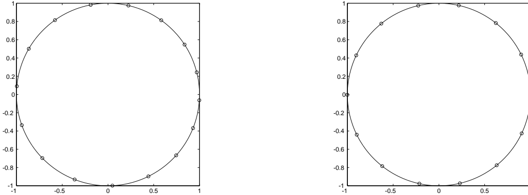
Figure 9: N = 16 approximate Fekete points of degree n = 15 in the complex disk of Example 4, with \varepsilon = 1 (left) and \varepsilon = 0.01 (right).
