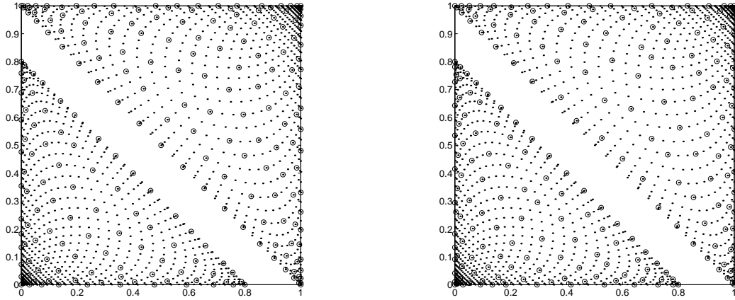
Figure 22: N = 231 approximate Fekete points of degree n = 20 (circles) extracted from a geometric weakly admissible mesh (dots) for Example 9-(40) with w_1 = 1, w_2 = 1 (left) and w_1 = 10, w_2 = 1 (right).
