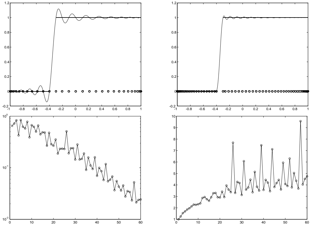
Figure 14: Top: high-pass polynomial nonweighted filters for K_1 = [-1, -0.4] and K_2 = [-0.3, 1] of degree n = 30 (left), and n = 60 (right); the small circles (o) indicate the approximate Fekete points. Bottom: interpolation errors (left) and Lebesgue constants (right) versus the interpolation degree.
