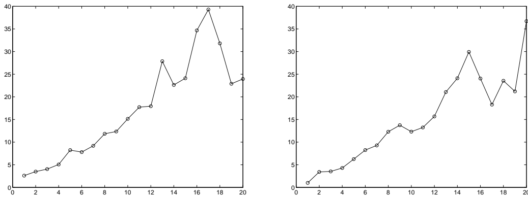
Figure 23: Estimated Lebesgue constants versus the interpolation degree for the two filters of Example 9-(40) with w_1 = 1, w_2 = 1 (left) and w_1 = 10, w_2 = 1 (right).
