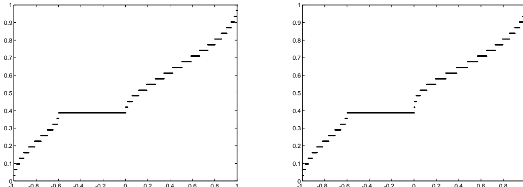
Figure 7: Distribution functions of N = 31 approximate Fekete points of degree n = 30 in Example 3, for \varepsilon = 0.3 (left) and \varepsilon = 0.01 (right).
