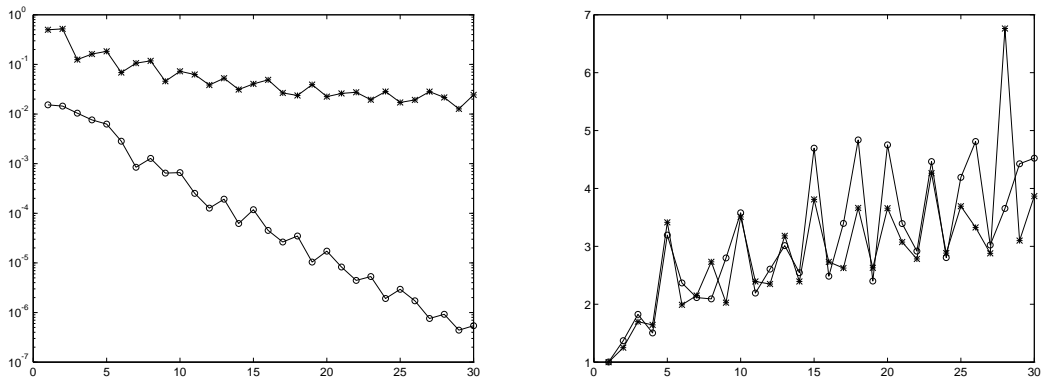
Figure 12: Interpolation errors (left) and Lebesgue constants (right) versus the interpolation degree, in Example 6; the interpolation spaces are \mathbb{P}_n with approximate Fekete points for nonweighted polynomial interpolation (*), and w\mathbb{P}_n with approximate Fekete points for weighted polynomial interpolation ( \circ ).
