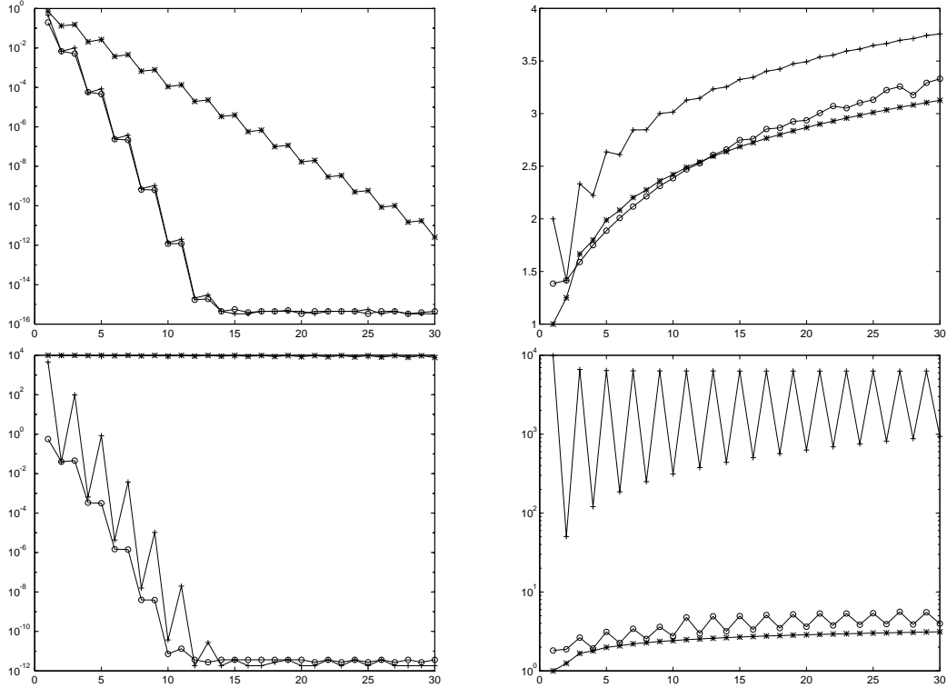
Figure 2: As in Figure 1 for the function of Example 2.
