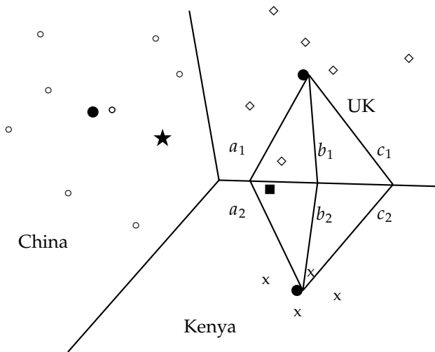
Figure 14.3 Rocchio classification.
