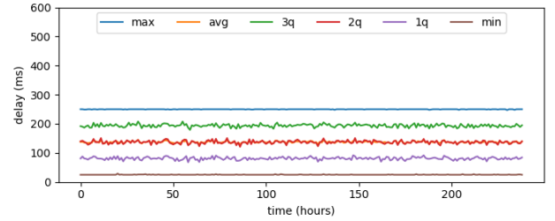
(b) Network delay of the sender-oriented approach.
