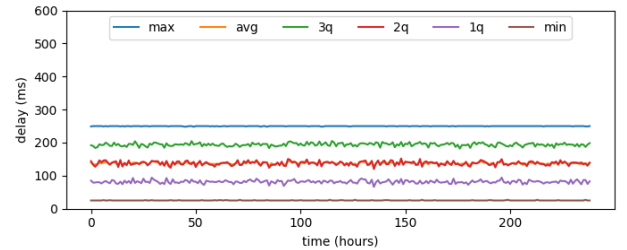
(c) Network delay of the receiver-oriented approach.
