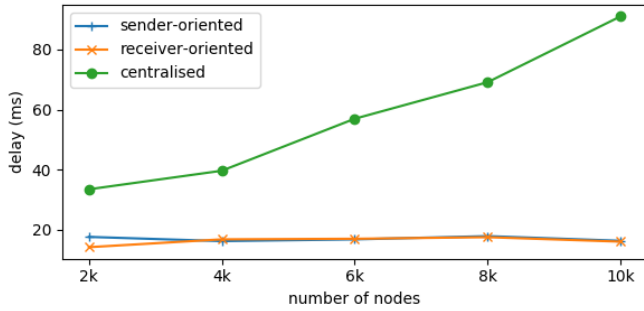
Figure 13: Comparison of the delays registered during the last hour of the simulation for an increasing number of simulated nodes.
