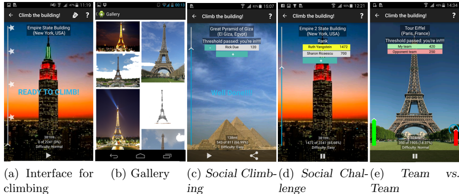
Fig. 1: ClimbTheWorld application.
