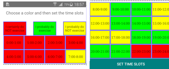
Fig. 2: Initial setup of time slots to provide initial information to the algorithm
