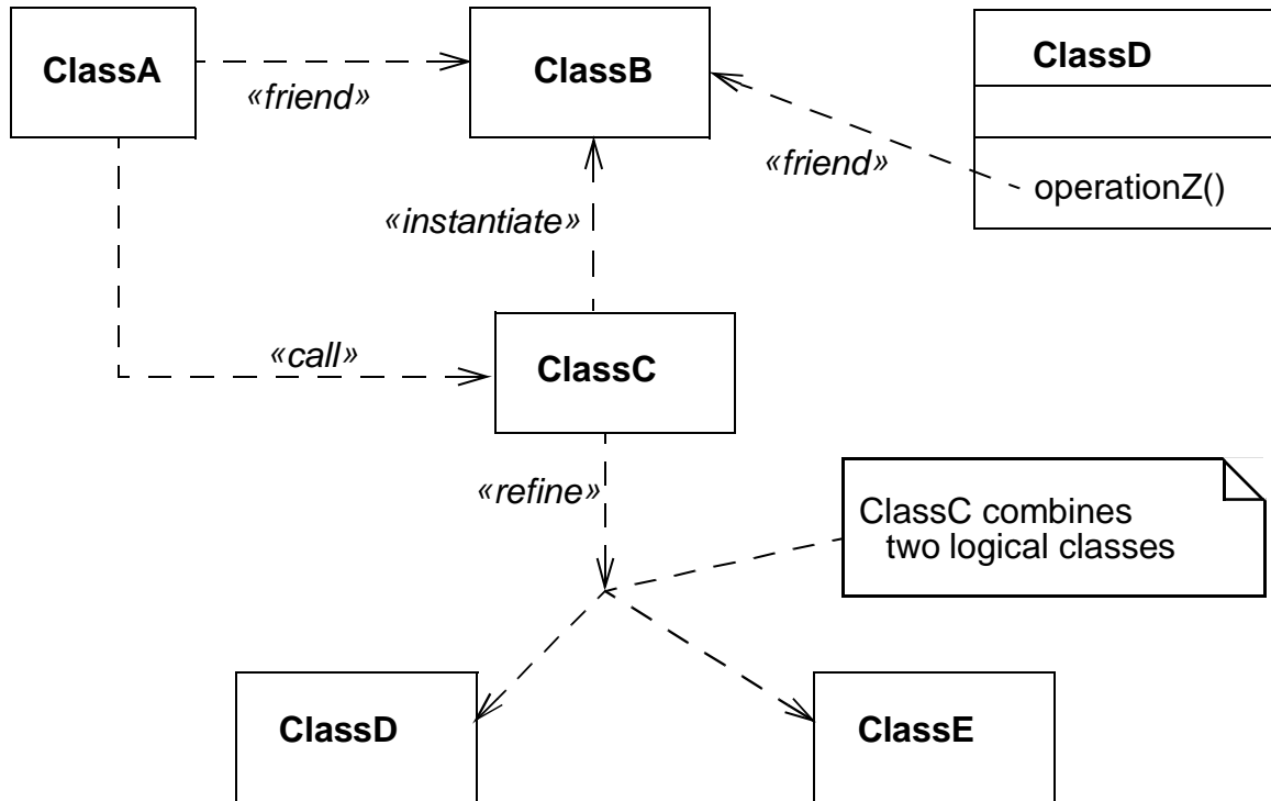
Figure 3-50 Various Dependencies Among Classes
