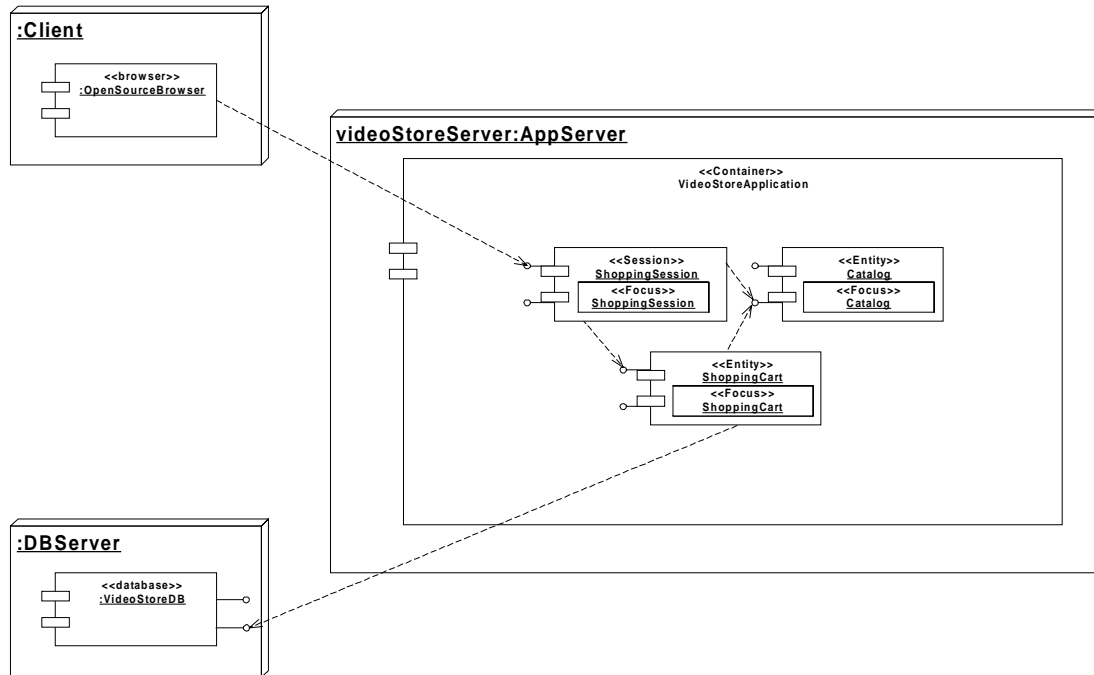
Figure 3-96 Deployment Diagram
