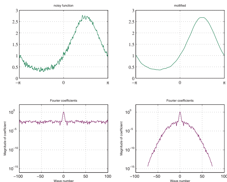
FIG. 8. Circular convolution of a noisy function with a smooth mollifier.
