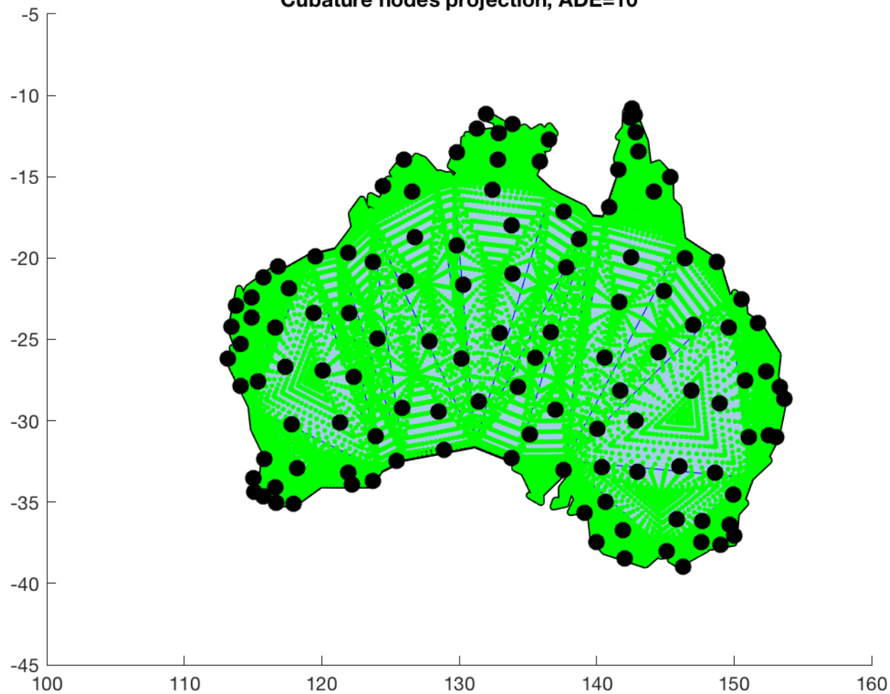
Cubature nodes projection, ADE=10
