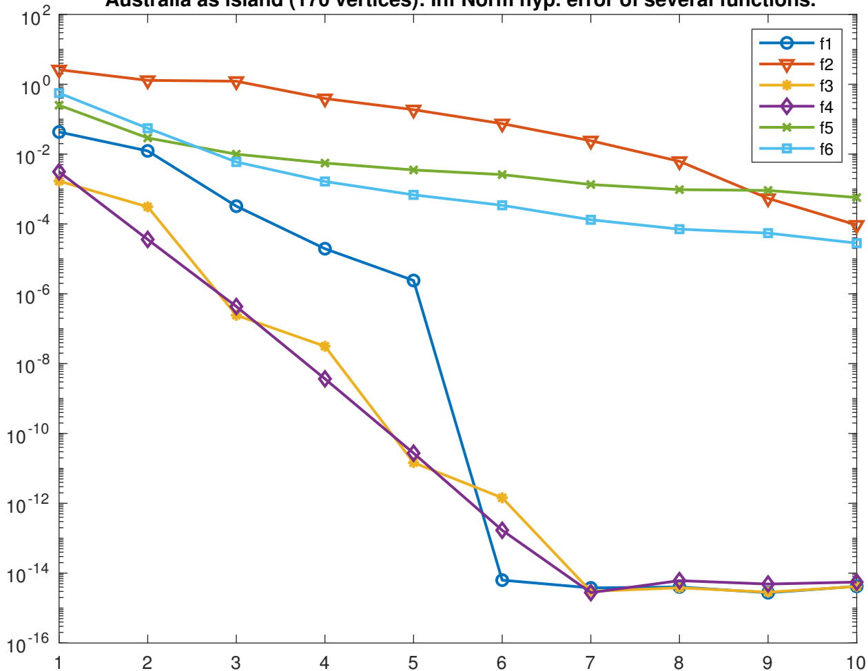
Australia as island (170 vertices): Inf Norm hyp. error of several functions.
