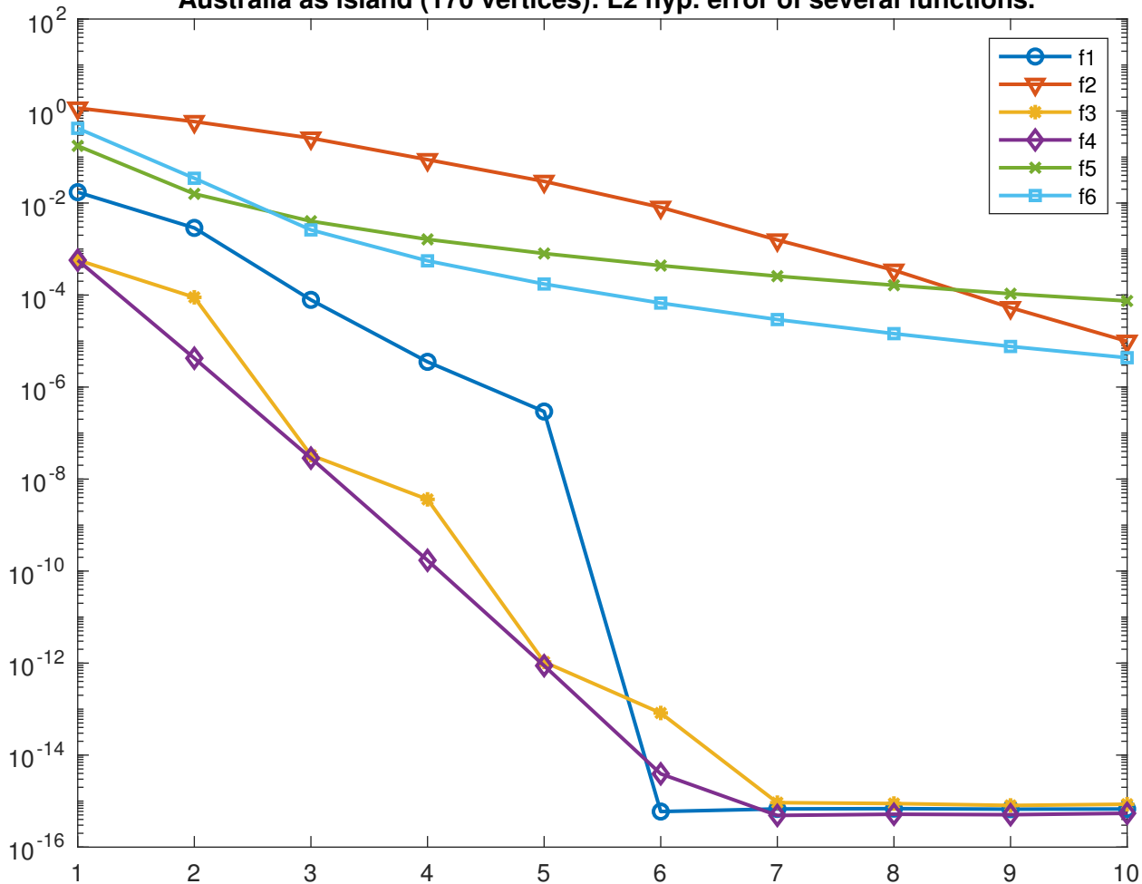
Australia as island (170 vertices): L2 hyp. error of several functions.
