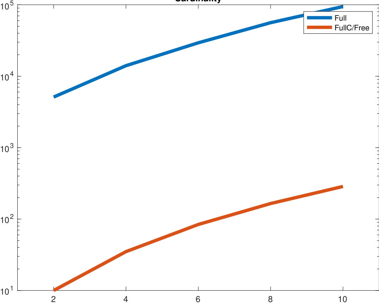
Cardinality
