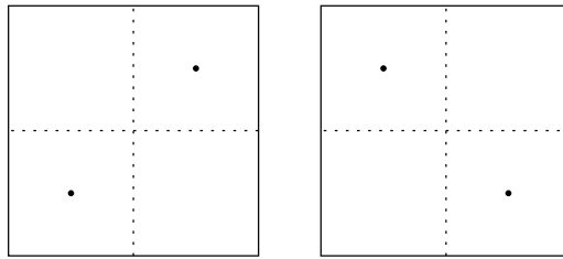
Figure 4.17 Configurations of two successive points.
