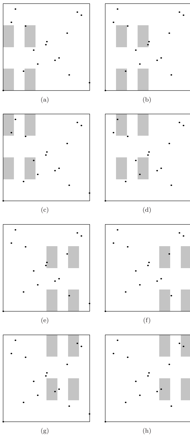
Figure 15.3 The digital (3, 2, 1, 8 \times 4, 2) -net. The union of the shaded rectangles in each figure from (a) to (h) contains exactly two points.
