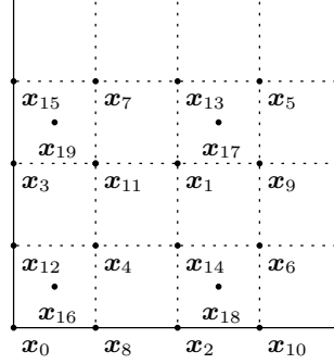
Figure 4.20 Construction of x_0, \dots, x_{19} .
