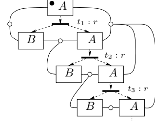
Fig. 6. A fragment of the unfolding of the graph grammar \mathcal{S} of Fig. 5.
