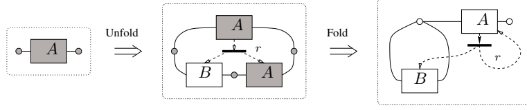
Fig. 7. An unfolding and a folding step for the graph grammar \mathcal{S} in Fig. 5.
