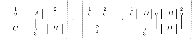
Fig. 4. A DPO rule corresponding to the rule in Fig. 2.
