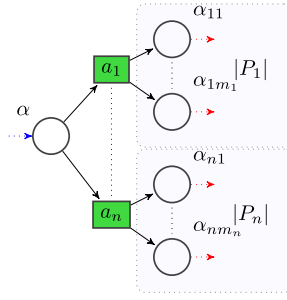
Fig. 24. Subnet corresponding to the process \oplus_{i=1}^n a_i.P_i .
