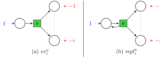
Fig. 16. The constant nets ev_i^a and repl_i^a .
