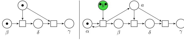
Fig. 14. Encodings for the processes (va)(a.a.nil \mid \bar{a}) and (lb.(va)(a.a.nil \mid \bar{a})) \mid \bar{b} \mid \bar{b} .
