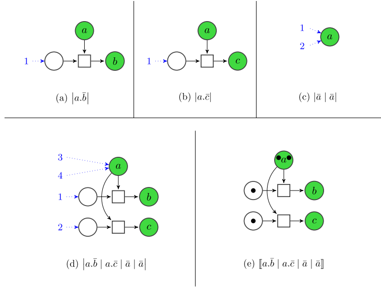
Fig. 12. The encoding of the process a.\bar{b} \mid a.\bar{c} \mid \bar{a} \mid \bar{a} .
