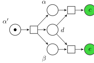
Fig. 13. Net encoding of the process (vd)(\tau.(d.\bar{c} \mid d.\bar{e} \mid \bar{d})) .
