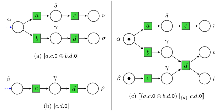
Fig. 18. Some process encodings.
