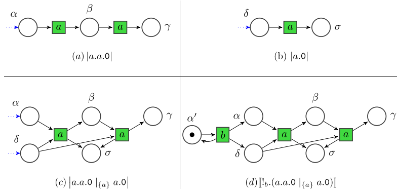
Fig. 19. Process encodings.
