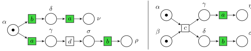
Fig. 20. Encoding for a.(d.b.nil \setminus d) \oplus b.a.nil and (c.a.nil |_{[c]} c.b.nil) \setminus c .
