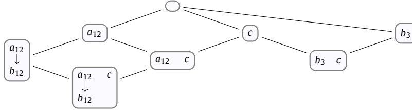
Fig. 2. Some prime event structures.
