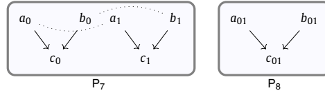
Fig. 10. Abstraction homomorphisms vs folding morphisms.
