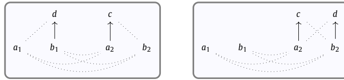
Fig. 9. Two PESS involved in the absorption law.
