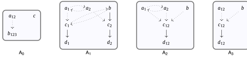
Fig. 4. Some asymmetric event structures.
