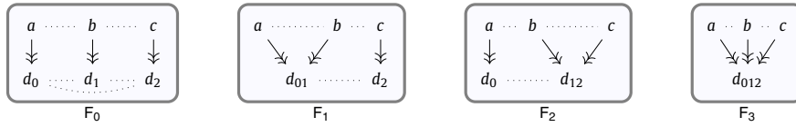
Fig. 5. Some flow event structures.
