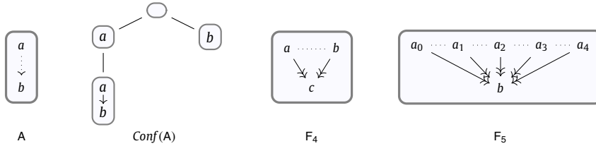
Fig. 6. Separating examples for AES, FESS, BESS.
