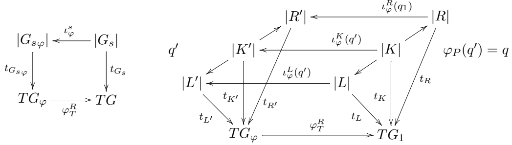
Figure 6.3: Graph processes.
