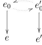
Figure 3.3: A pre-AES with two conflictual events e and e' , not related by asymmetric conflict.
