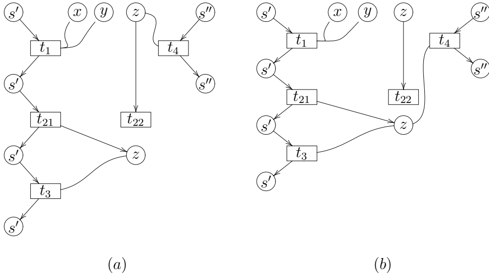
Figure 1.4: The contextual net processes for two possible schedulings of the transactions T' and T'' .
