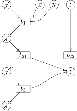
Figure 1.3: The contextual net process corresponding to a transaction.
