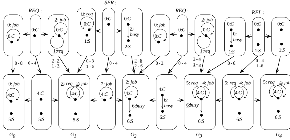
Figure 5.5: A derivation of grammar \mathcal{G} starting from graph G_0 .
