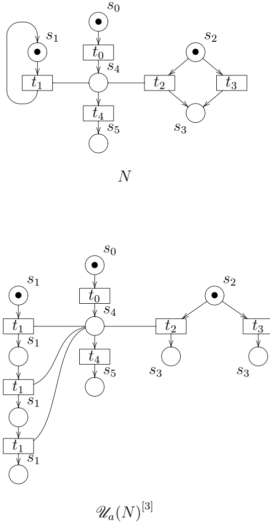
Figure 3.5: A c-net and (part of ) its unfolding.
