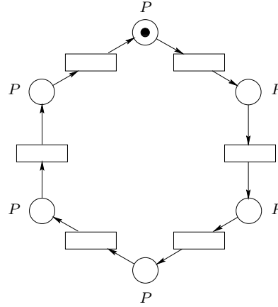
Figure 1.8: A Petri net representation of system RING.
