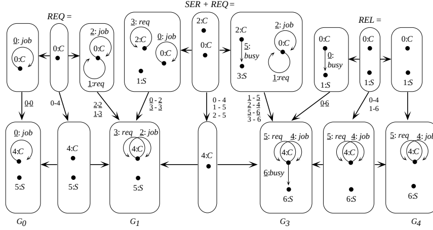
Figure 5.11: A derivation \rho' in grammar \mathcal{C}\text{-}\mathcal{S} , shift-equivalent to derivation \rho of Figure 5.6.
