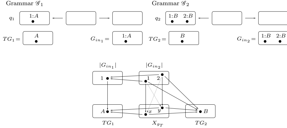
Figure 6.6: The grammars \mathcal{G}_1 and \mathcal{G}_2 , and the pullback-retyping diagram for their start graphs.
