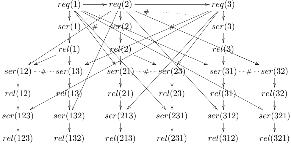
Figure 8.1: Event structure of the grammar \mathcal{C}\text{-}\mathcal{S} .
