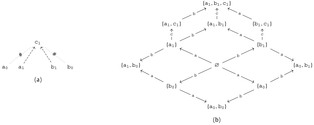
Fig. 1. (a): The configuration structure C_1 and (b) its transition system.
