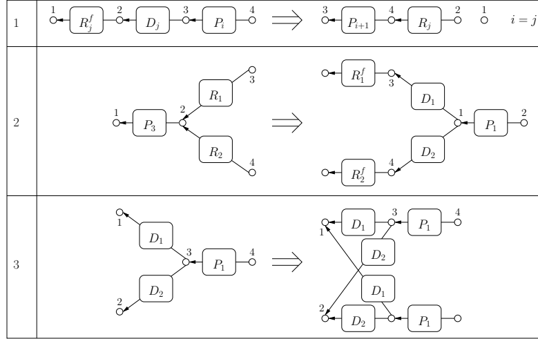
Fig. 2. Rewriting rules of the GTS Sys.
