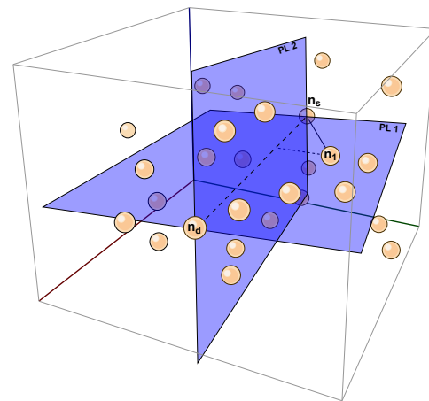
Fig. 3. In AB3D, plane PL_1 passes through n_s , n_d and n_1 , plane PL_2 is orthogonal to PL_1 . Both planes contain the line (n_s n_d)
