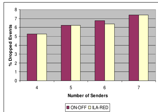
Figure 16. Percentage of discarded events; AIDT = 60ms.
