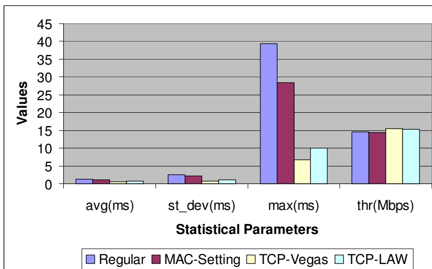
Figure 62. Statistical values for the various schemes.
