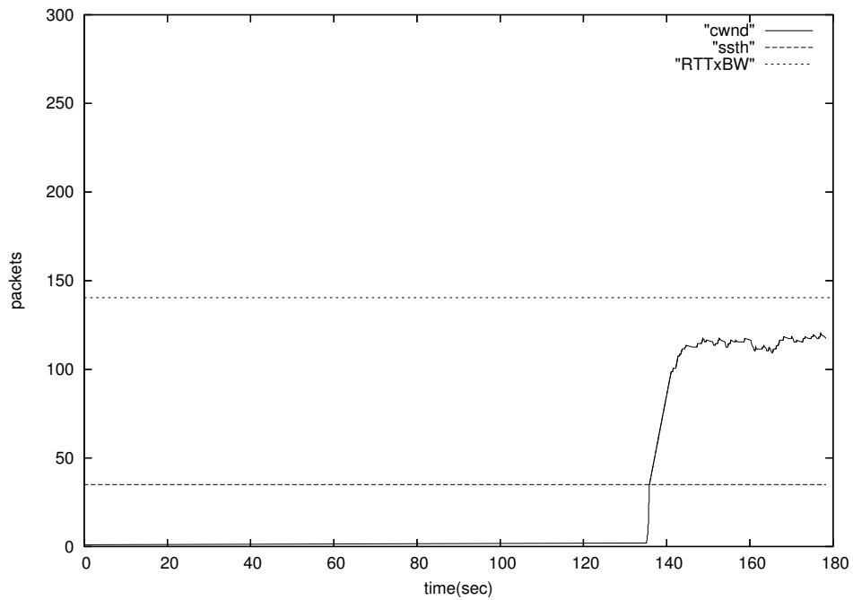
Figure 55. TCP Vegas congestion window; \alpha = 1 , \beta = 3 , \gamma = 2 .
