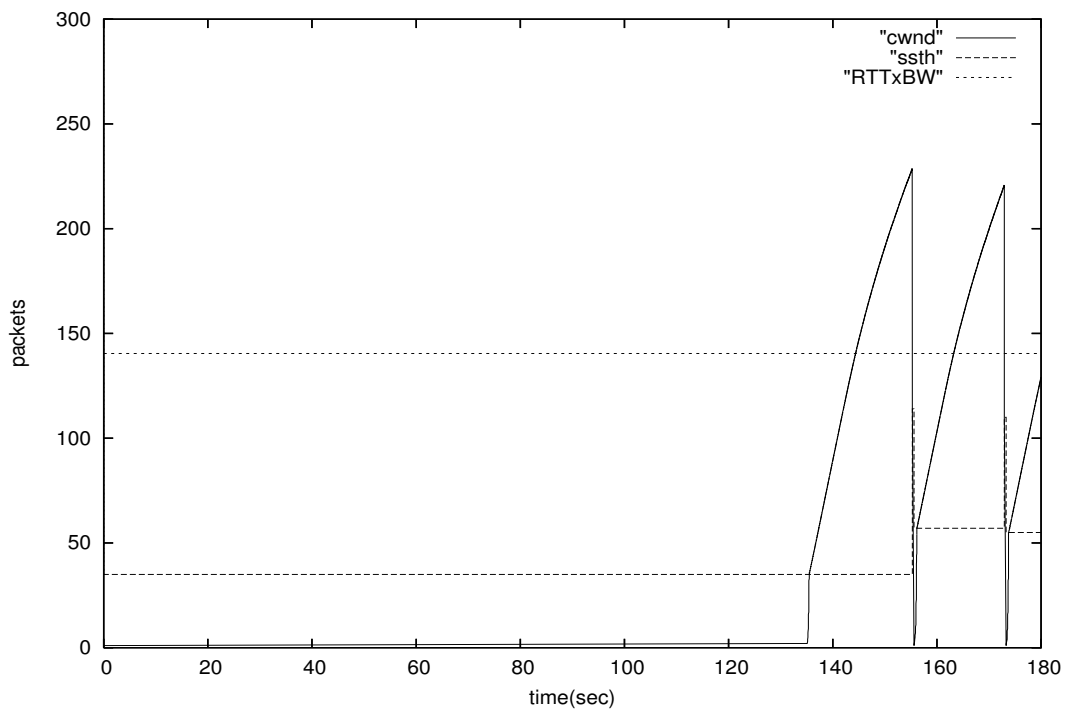
Figure 47. TCP congestion window; MAC max retransmissions = 4, buffer size = 50 packets.
