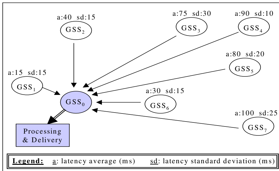
Figure 8. The adopted configuration.
