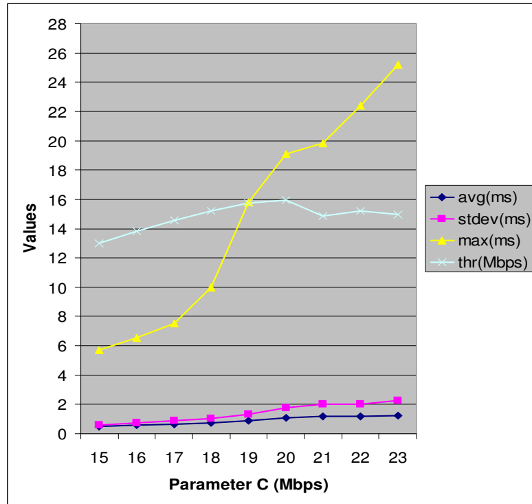
Figure 58. Statistical values when employing limited advertised window.
