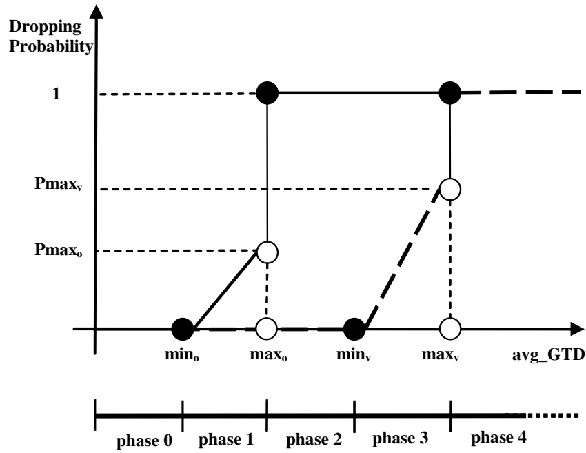
Figure 6. Discarding probability functions for ILA-RIO.
