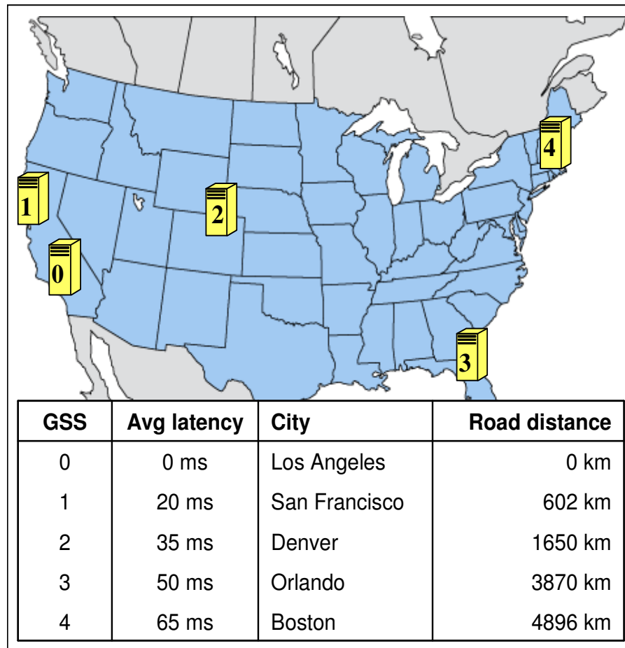
Figure 22. Game servers deployment.
