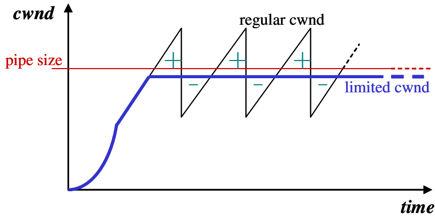
Figure 36. Comparison between regular and limited sending windows.
