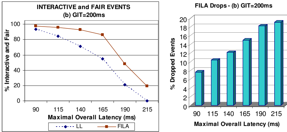
Figure 24. Interactivity and fairness improvement (left) and dropped events (right) with GIT=200ms and AIDT=30ms.
