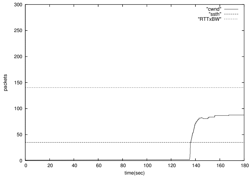
Figure 50. TCP Vegas congestion window; \alpha = 1 , \beta = 3 , \gamma = 2 .
