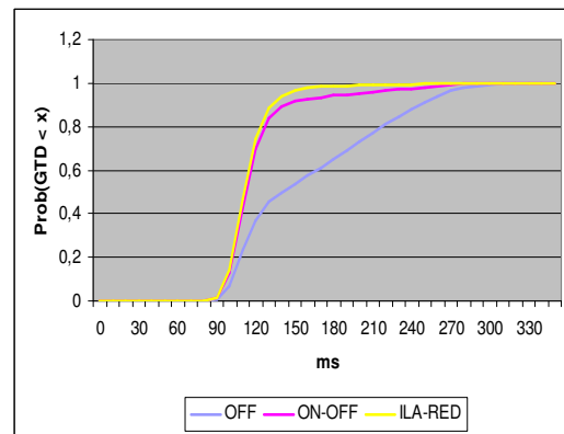
Figure 10. Cumulative function of the GTDs in a scenario with 7 GSSs; AIDT = 30ms.
