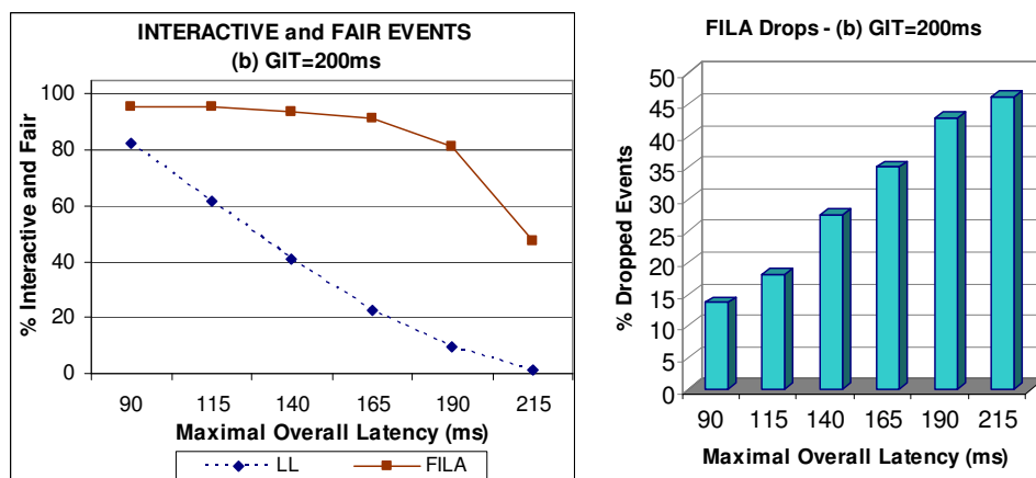
Figure 32. Interactivity and fairness improvement (left) and dropped events (right) with GIT=200ms and AIDT=10ms.
