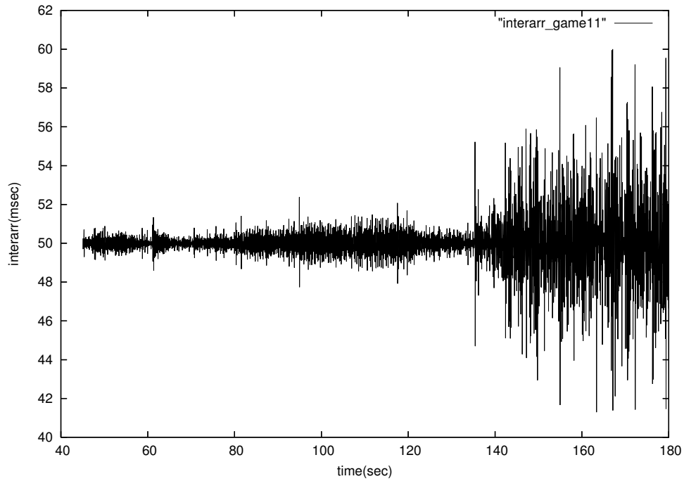
Figure 60. Online game interarrival time with concurrent TCP, limited advertised window, C = 18\text{Mbps} .
