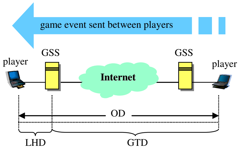
Figure 21. Delay definitions.
