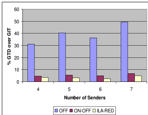
Figure 9. Percentage of events with GTD over GIT; AIDT = 30ms.
