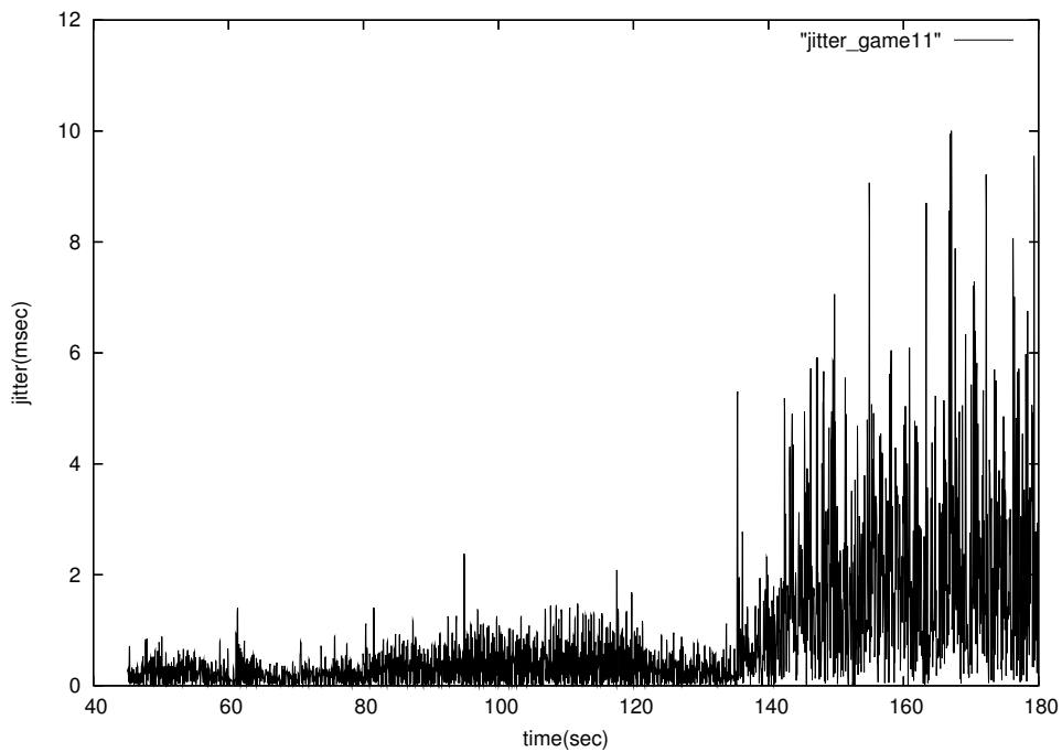
Figure 61. Online game jitter with concurrent TCP, limited advertised window, C = 18\text{Mbps} .
