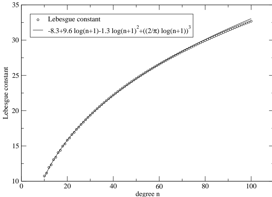
Figure 1: The Lebesgue constant of hyperinterpolation in the cube up to degree 100.
