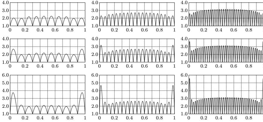
Fig. 1 Lebesgue function of the Floater–Hormann interpolants for d = 1 (top), d = 2 (middle), and d = 3 (bottom) at n + 1 equidistant nodes for n = 10, 20, 40 .
