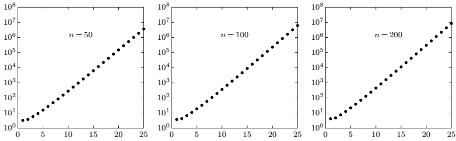
Fig. 4 Lebesgue constants of the Floater–Hormann interpolants at a fixed number of n + 1 equidistant nodes for 1 \leq d \leq 25 .
