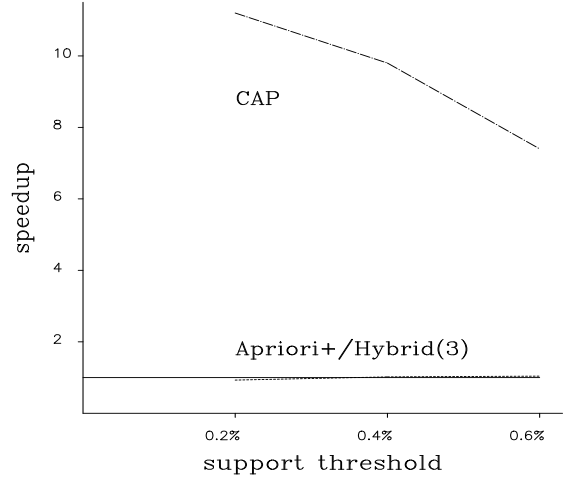
(b) Speedup vs Support
