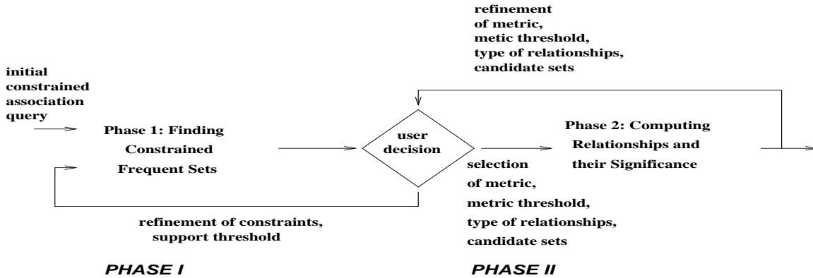
Figure 1: An Architecture for Exploratory Association Mining
