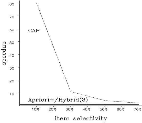
(a) Speedup vs Selectivity
