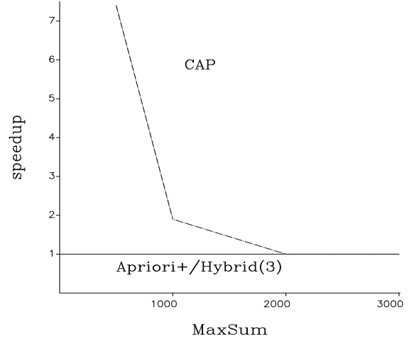
(b) Anti-monotone, Non-succinct
