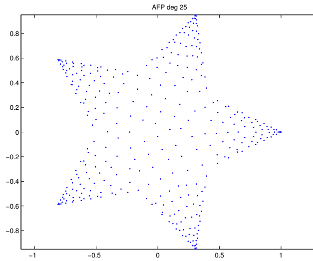
FIGURE 6.2.2. Approximate Fekete points of degree 25 for the star shape, extracted from the admissible mesh of Figure 6.1.1.
