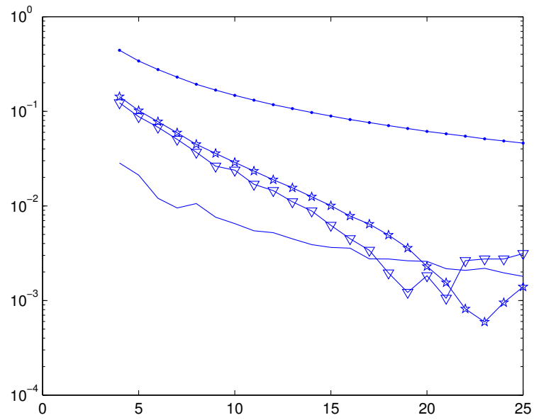
FIGURE 6.4.7. The approximation of the L^1([-5, 5]^2 \setminus \bar{\mathbb{S}}^2) relative errors of the approximation of V_{\bar{\mathbb{S}}^2}^* by V_{E,k}^{(1)} (dots and line), V_{E,k}^{(2)} (line), V_{E,k}^{(3)} (stars and line), and V_{E,k}^{(4)} (triangles and line).
