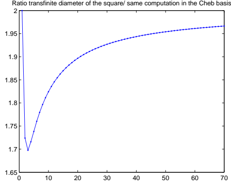
FIGURE 6.4.3. Numerical computation of the factor \frac{1}{2} \left( \frac{1}{\det \tilde{G}_k(\hat{\mu}_k)} \right)^{\frac{n+1}{2nkN_k}} for (6.4.2).
