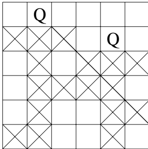
Figure 1: A search state in the 6-queens problem
