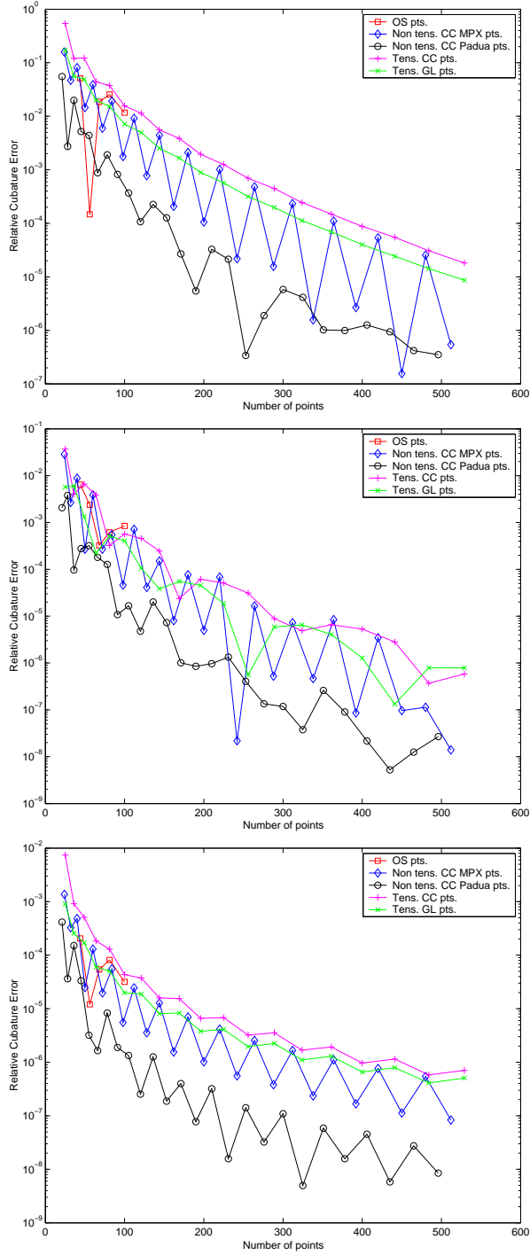
Figure 2: Relative cubature errors versus the number of cubature points (CC = Clenshaw-Curtis, GL = Gauss-Legendre, MPX = Morrow-Patterson-Xu, OS = Omelyan-Solovyan) for the three test functions: f(\mathbf{x}) = 1/(1 + 16|\mathbf{x}|^2) (top), f(\mathbf{x}) = \exp(-1/|\mathbf{x}|^2) (center), f(\mathbf{x}) = |\mathbf{x}|^3 (bottom); the integration domain is [-1, 1]^2 , the integrals up to machine precision are, respectively: 0.597388947274307, 0.853358758654305 and 2.508723139534059.
