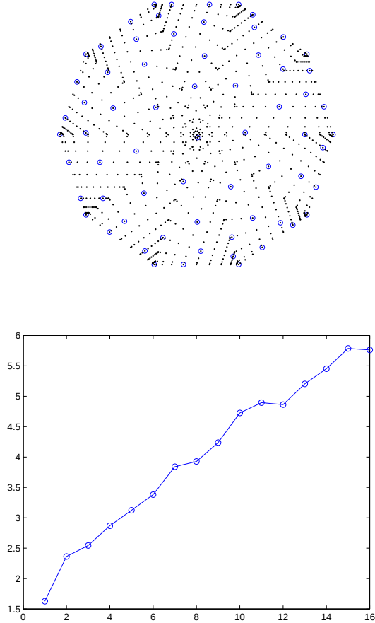
Figure 5: Top: WAM (dots) and corresponding approximate Fekete points (small circles) of degree 10 on a regular decagon. Bottom: norm of the least squares projection operator on approximate Fekete points of degree 2n , n = 1, \dots, 16 .
