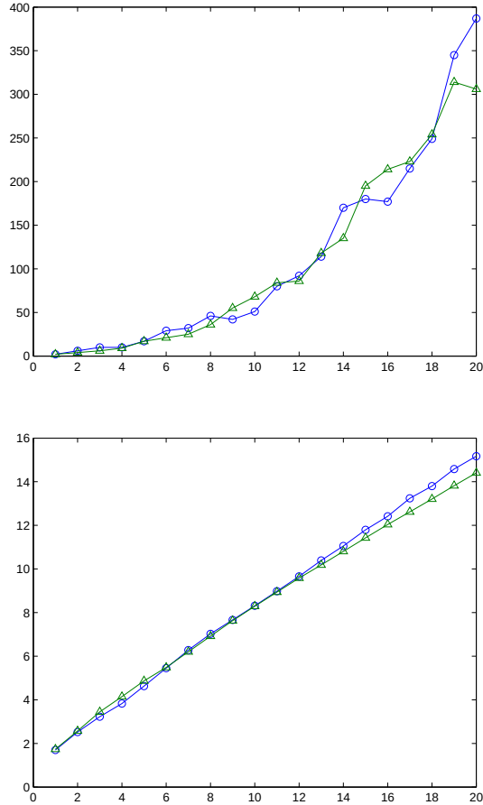
Figure 2: Lebesgue constants of the approximate Fekete points (top) and norms of the least squares approximation operators (bottom), for the WAMs of the pyramid (small triangles) and truncated cone (small circles) in Figure 1, at degree n = 1, \dots, 20 .
