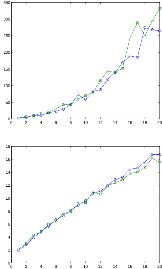
Figure 4: Lebesgue constants of the approximate Fekete points (top) and norms of the least squares approximation operators (bottom), for the WAMs of a portion of torus with circular section (small circles) and square section (small squares), at degree n = 1, \dots, 20 .
