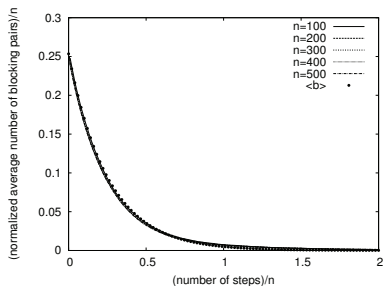
Figure 1. Convergence speed.
